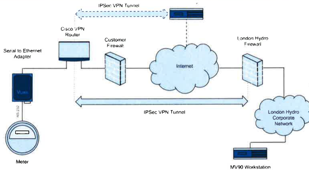
Figure 4-1, Internet Metering
